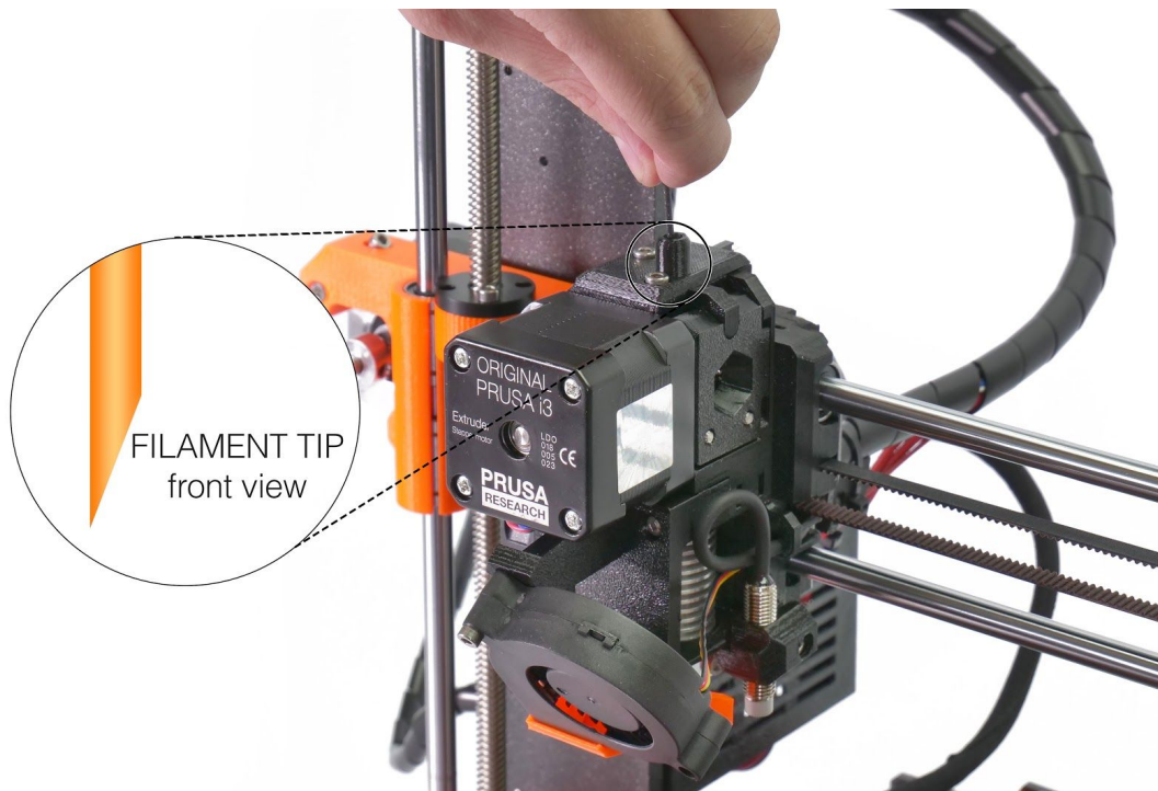
Pict. 9 - Loading the filament into the extruder
